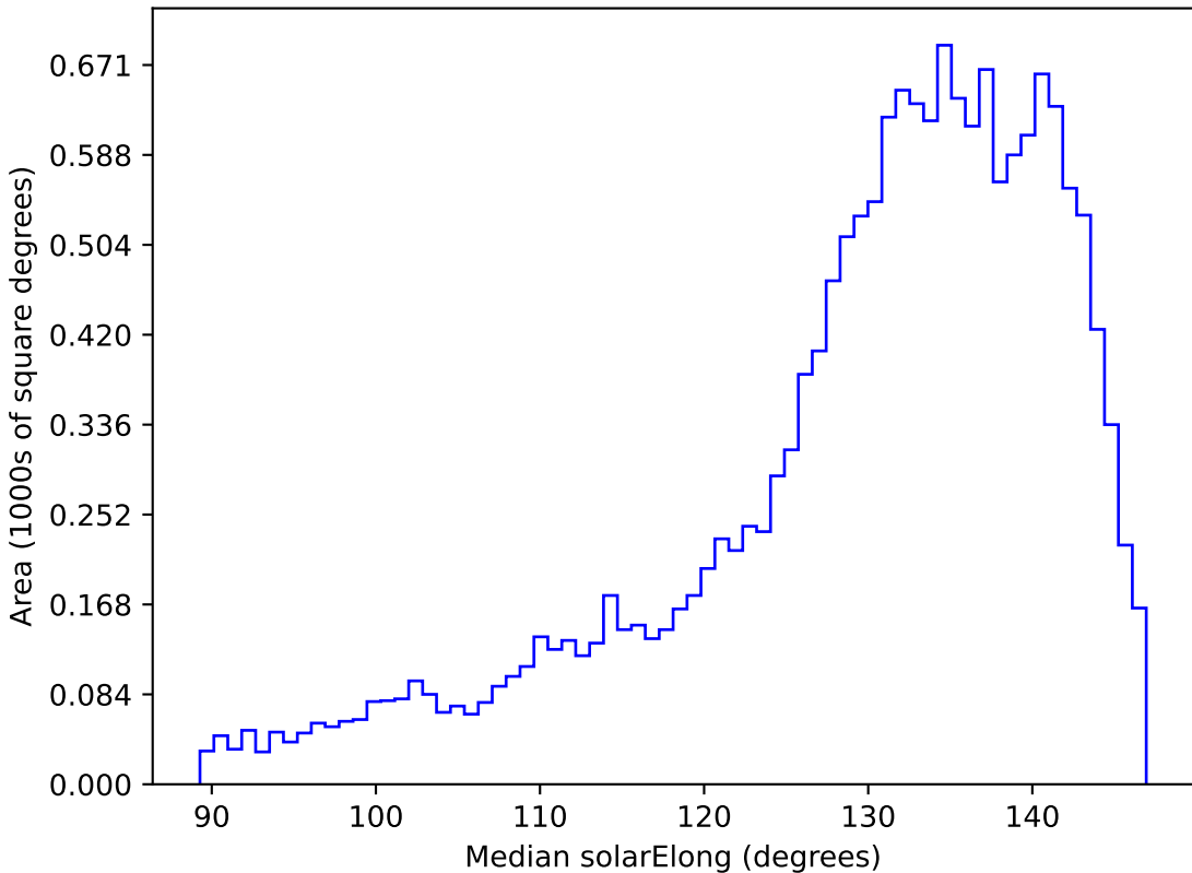
too_elab_r32_d3_griz_v3.4_10yrs WFD y band: Median solarElong
