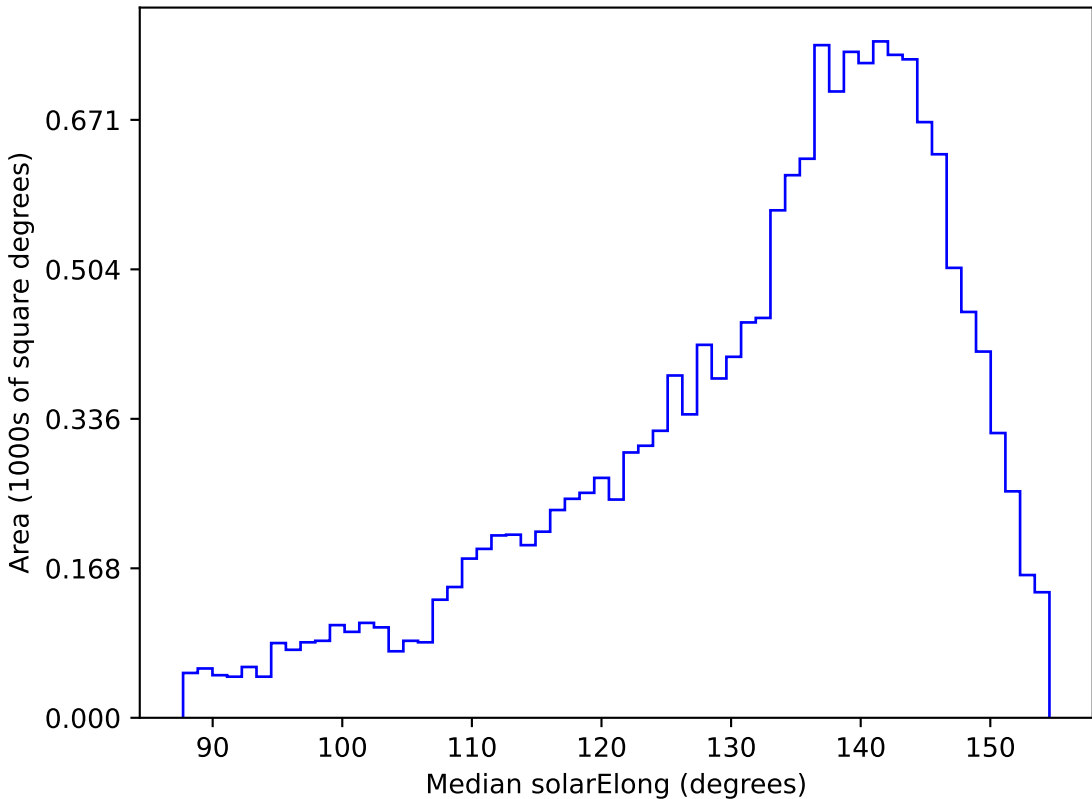
too_elab_r32_d3_griz_v3.4_10yrs WFD u band: Median solarElong
