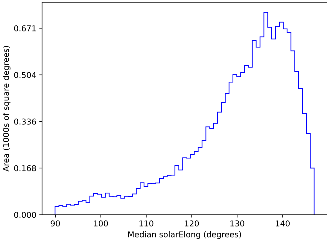
too_elab_r32_d3_griz_v3.4_10yrs WFD r band: Median solarElong
