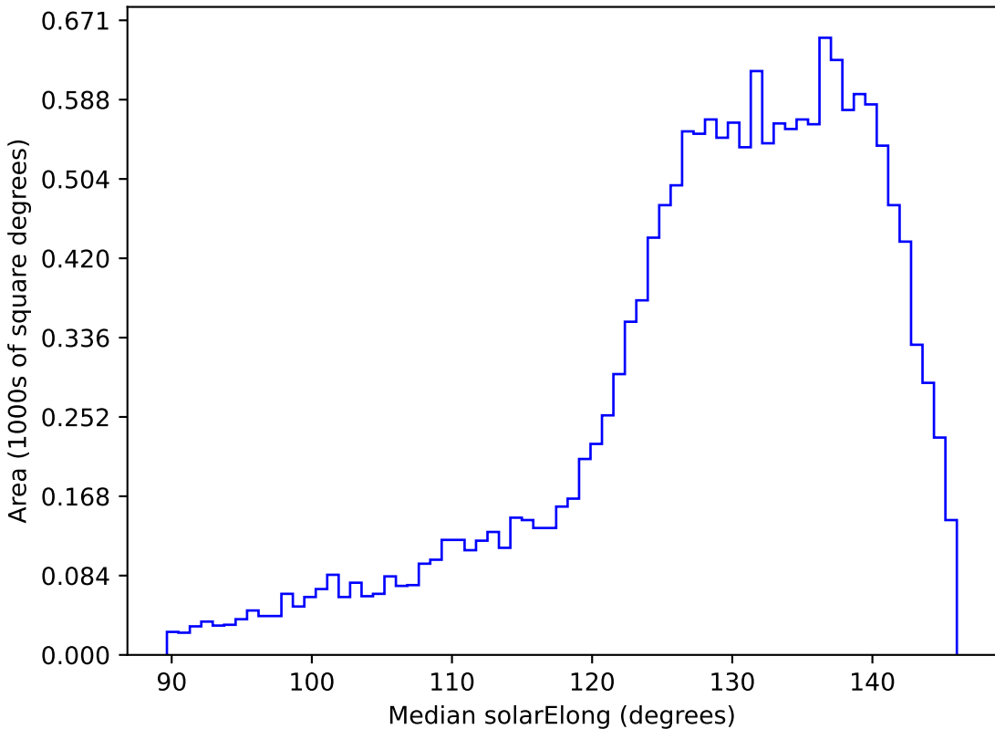
too_elab_r32_d3_griz_v3.4_10yrs WFD i band: Median solarElong
