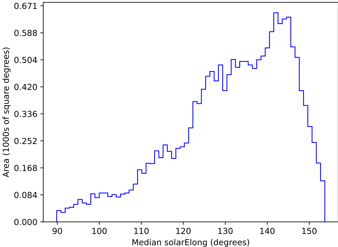
too_elab_r32_d3_griz_v3.4_10yrs WFD g band: Median solarElong
