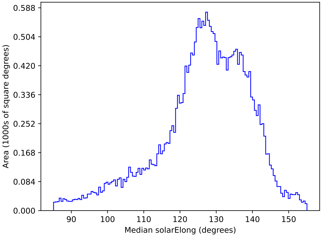
too_elab_r32_d3_griz_v3.4_10yrs All sky z band: Median solarElong
