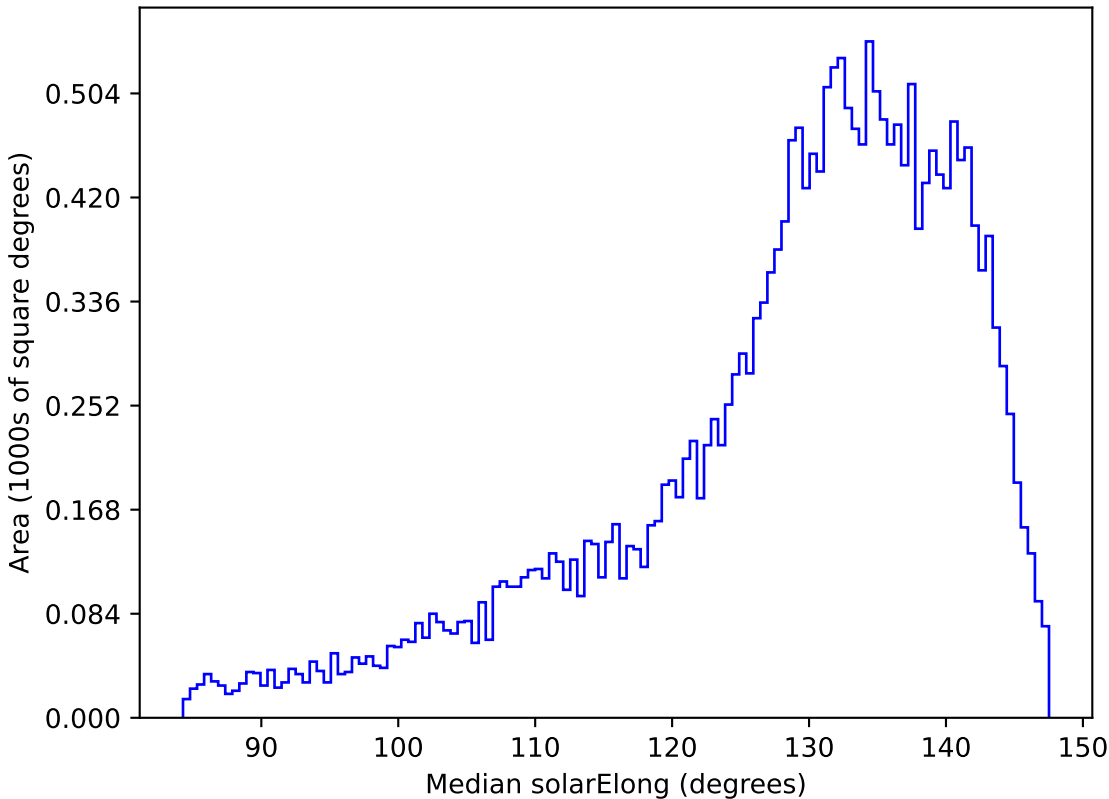
too_elab_r32_d3_griz_v3.4_10yrs All sky y band: Median solarElong
