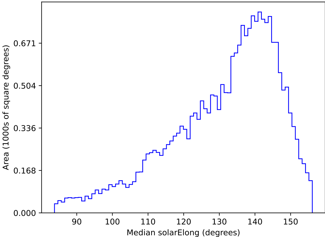
too_elab_r32_d3_griz_v3.4_10yrs All sky u band: Median solarElong
