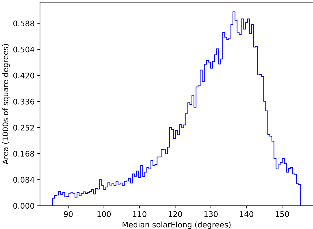
too_elab_r32_d3_griz_v3.4_10yrs All sky r band: Median solarElong
