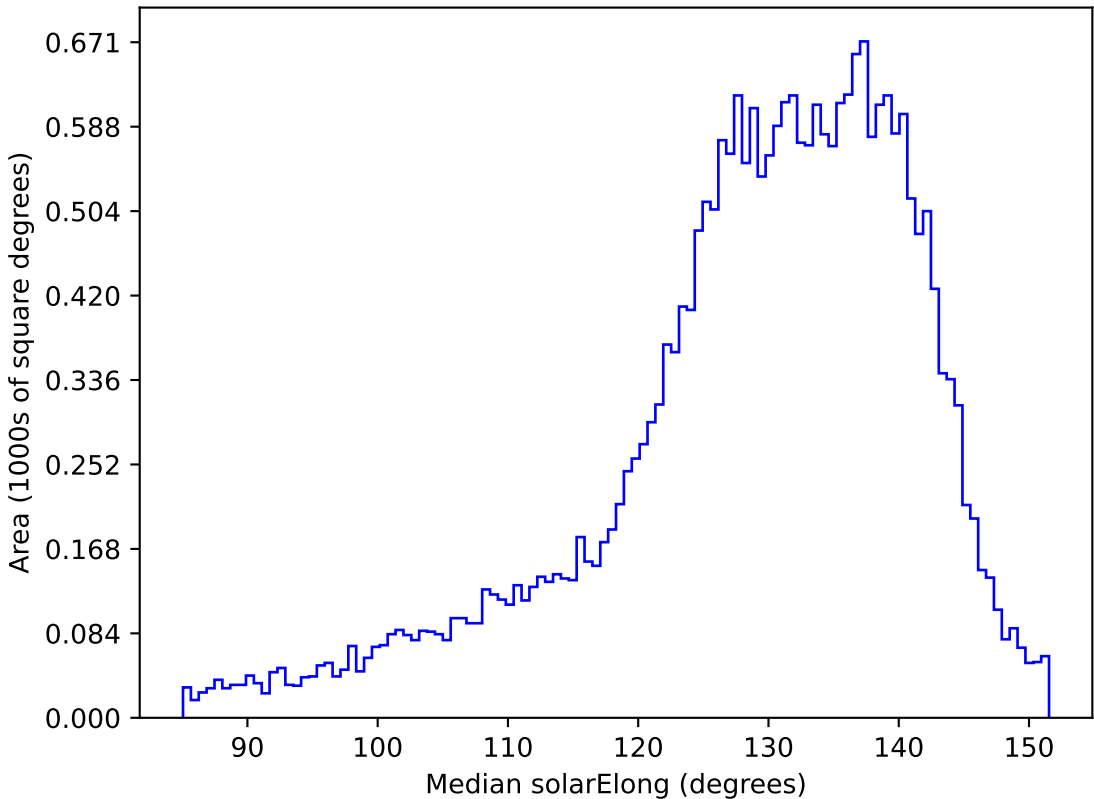
too_elab_r32_d3_griz_v3.4_10yrs All sky i band: Median solarElong
