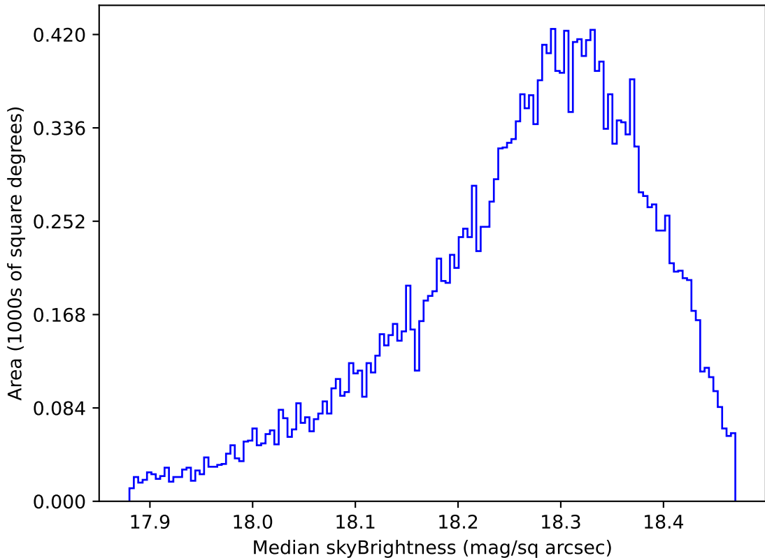
too_elab_r32_d3_griz_v3.4_10yrs Yr 1 y band: Median skyBrightness
