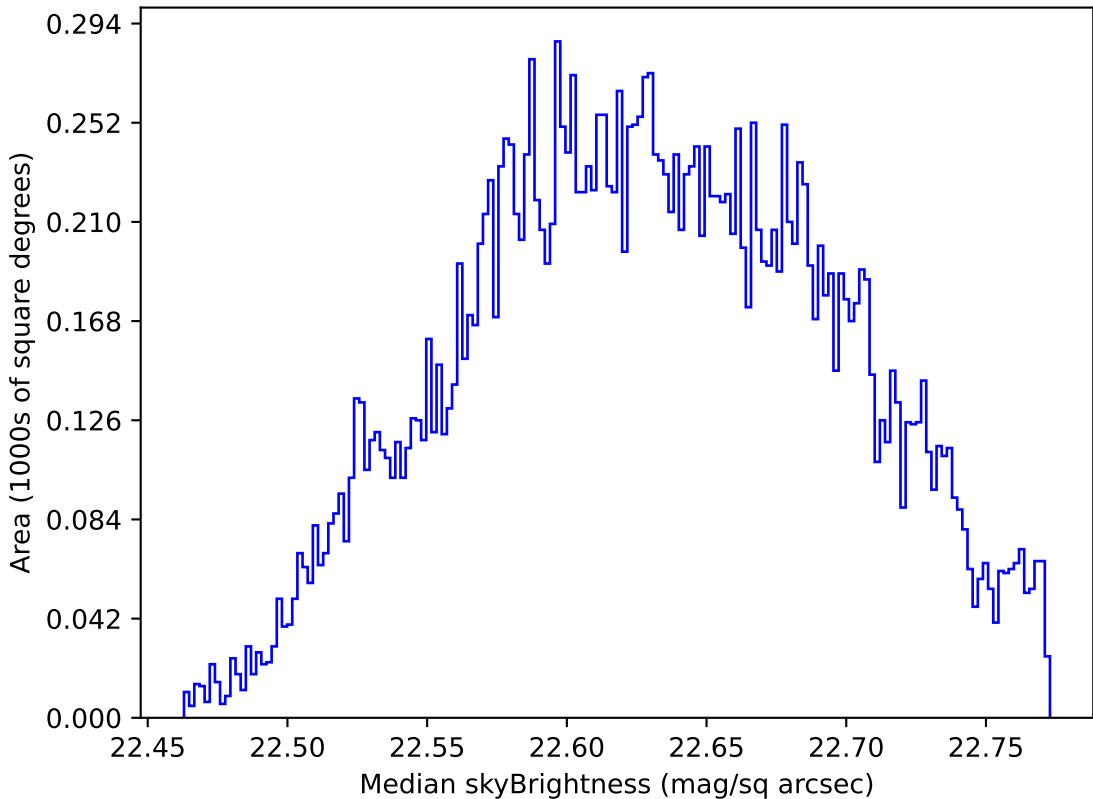
too_elab_r32_d3_griz_v3.4_10yrs Yr 1 u band: Median skyBrightness
