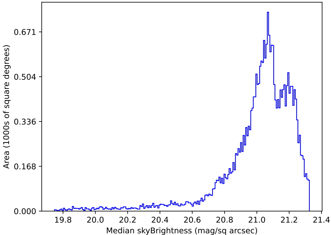
too_elab_r32_d3_griz_v3.4_10yrs Yr 1 r band: Median skyBrightness
