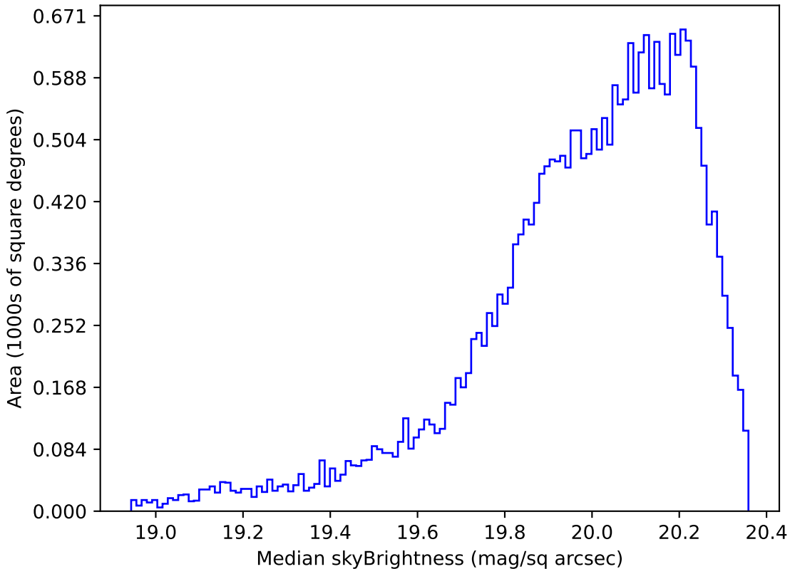
too_elab_r32_d3_griz_v3.4_10yrs Yr 1 i band: Median skyBrightness
