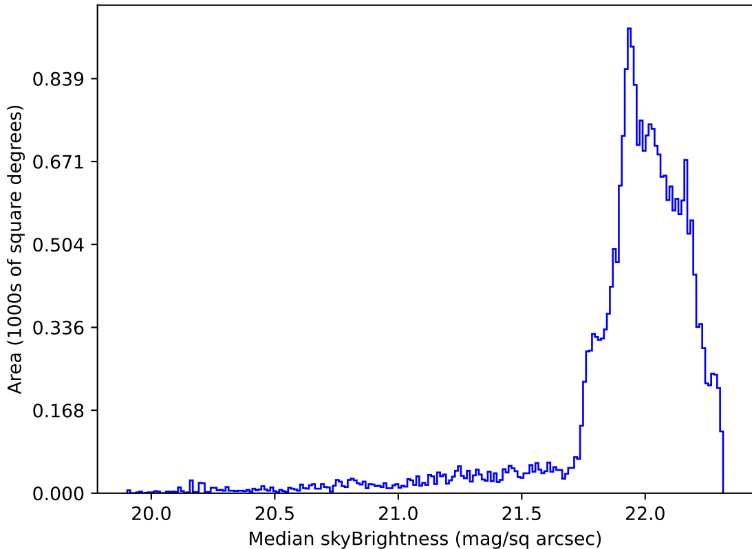
too_elab_r32_d3_griz_v3.4_10yrs Yr 1 g band: Median skyBrightness
