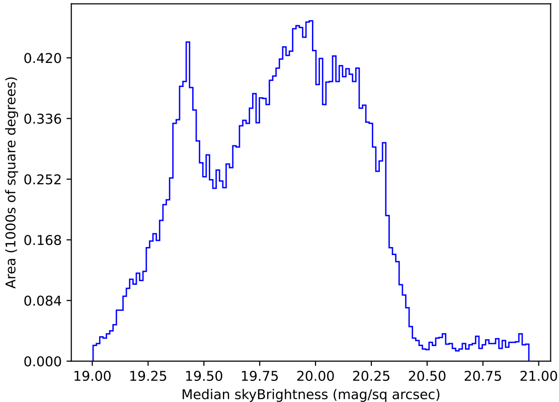
too_elab_r32_d3_griz_v3.4_10yrs Yr 1 all bands: Median skyBrightness
