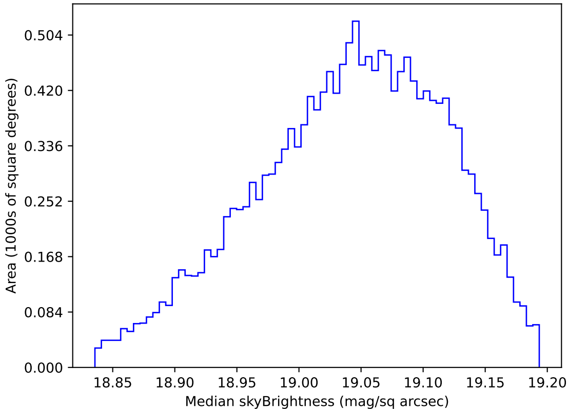
too_elab_r32_d3_griz_v3.4_10yrs WFD z band: Median skyBrightness
