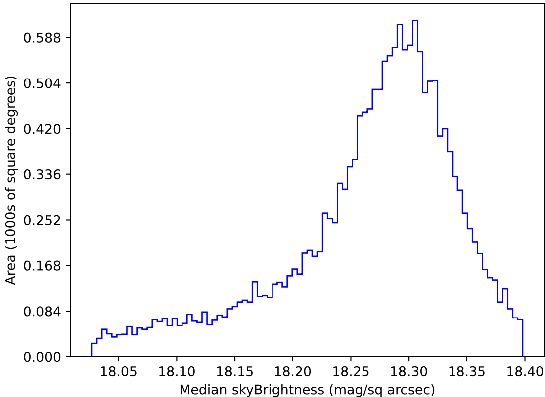
too_elab_r32_d3_griz_v3.4_10yrs WFD y band: Median skyBrightness
