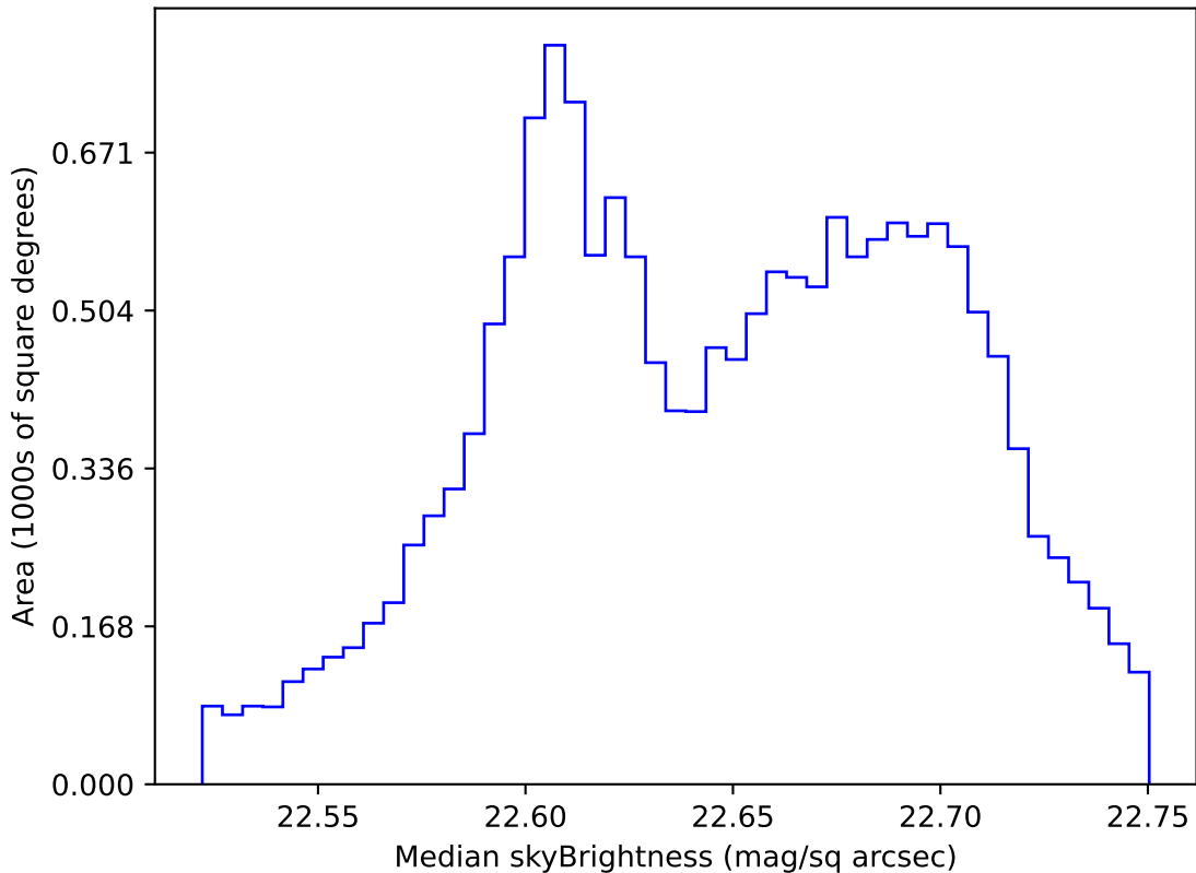
too_elab_r32_d3_griz_v3.4_10yrs WFD u band: Median skyBrightness
