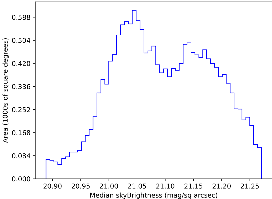
too_elab_r32_d3_griz_v3.4_10yrs WFD r band: Median skyBrightness
