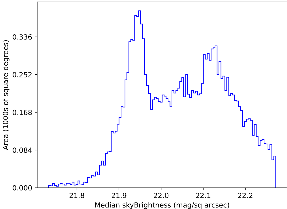
too_elab_r32_d3_griz_v3.4_10yrs WFD g band: Median skyBrightness
