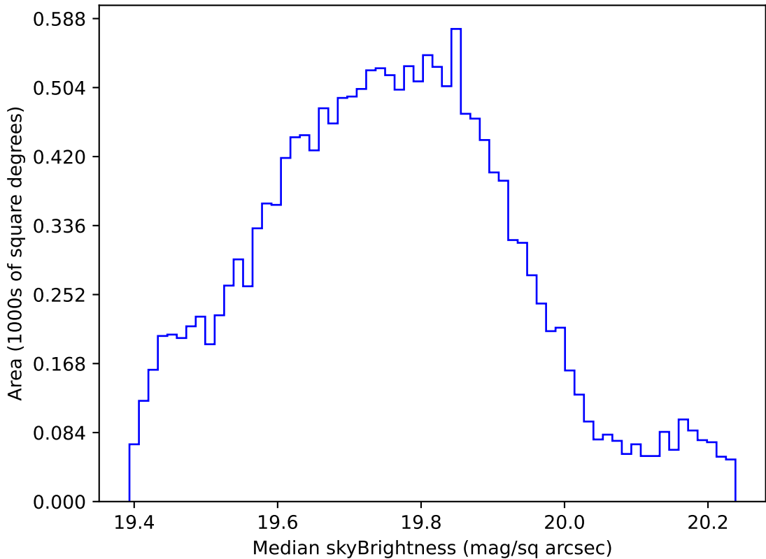
too_elab_r32_d3_griz_v3.4_10yrs WFD all bands: Median skyBrightness
