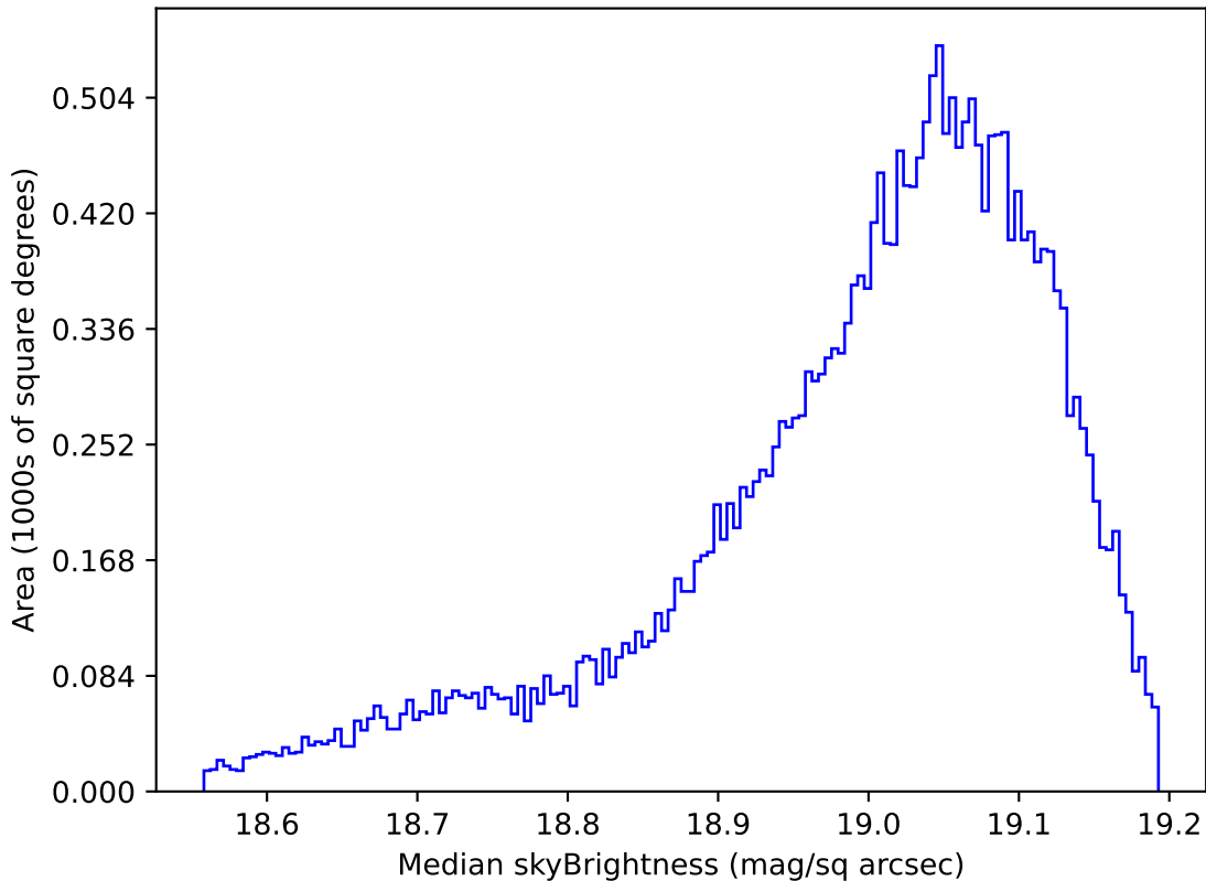
too_elab_r32_d3_griz_v3.4_10yrs All sky z band: Median skyBrightness
