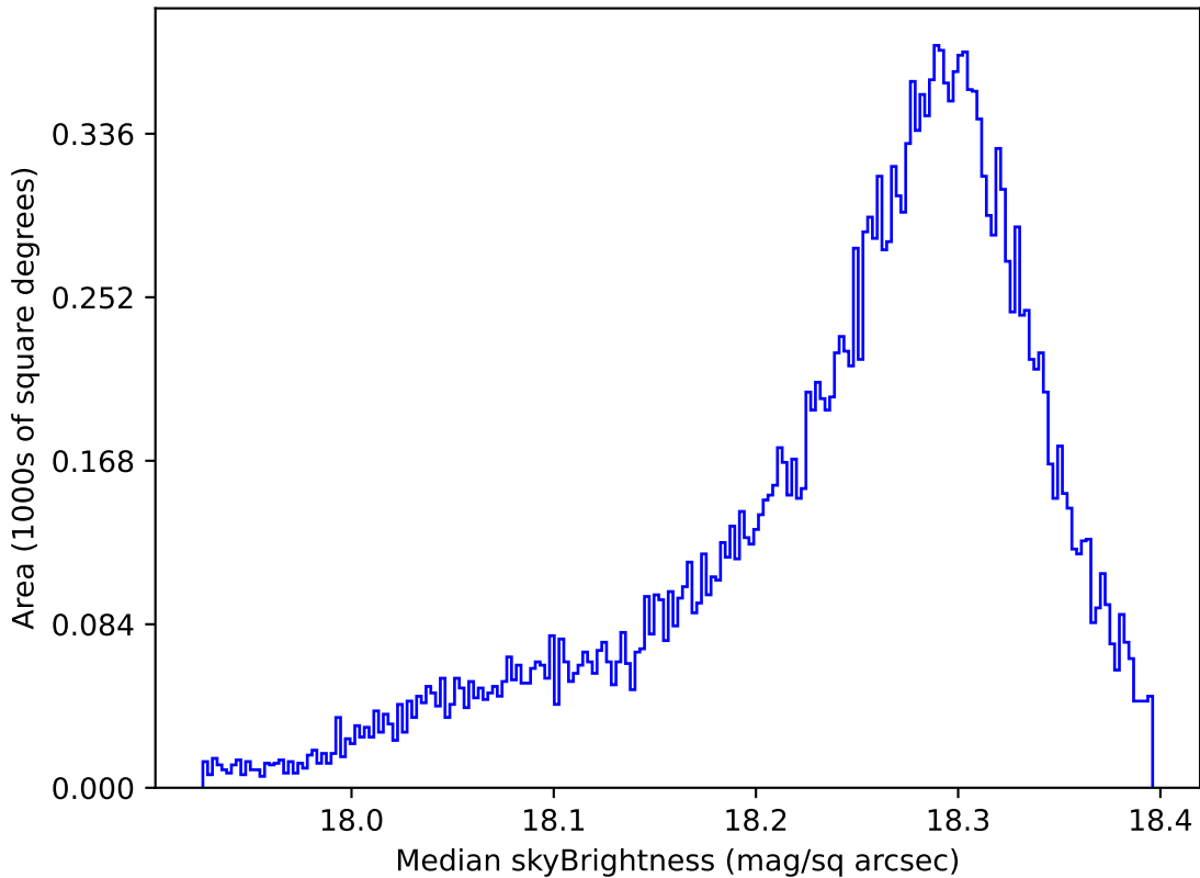
too_elab_r32_d3_griz_v3.4_10yrs All sky y band: Median skyBrightness
