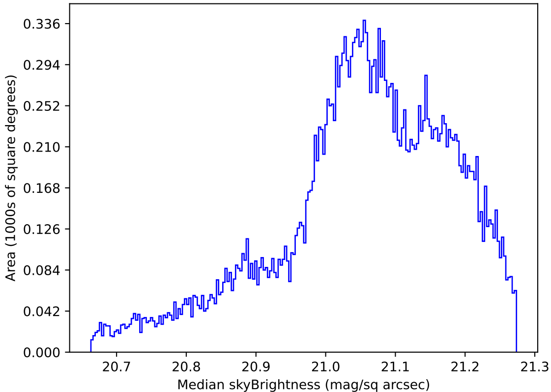
too_elab_r32_d3_griz_v3.4_10yrs All sky r band: Median skyBrightness
