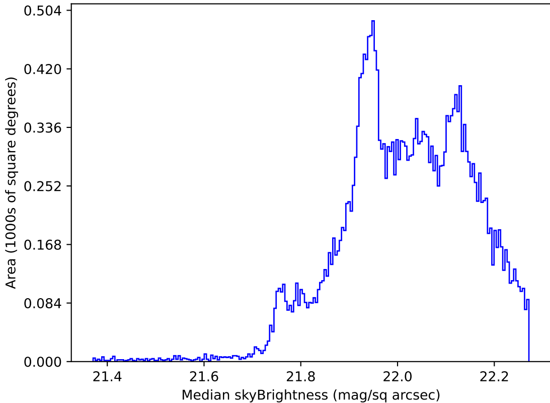
too_elab_r32_d3_griz_v3.4_10yrs All sky g band: Median skyBrightness
