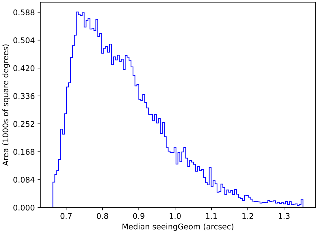
too_elab_r32_d3_griz_v3.4_10yrs Yr 1 r band: Median seeingGeom
