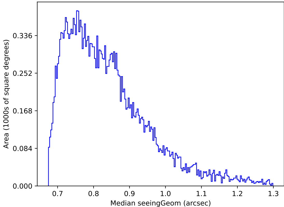
too_elab_r32_d3_griz_v3.4_10yrs Yr 1 i band: Median seeingGeom
