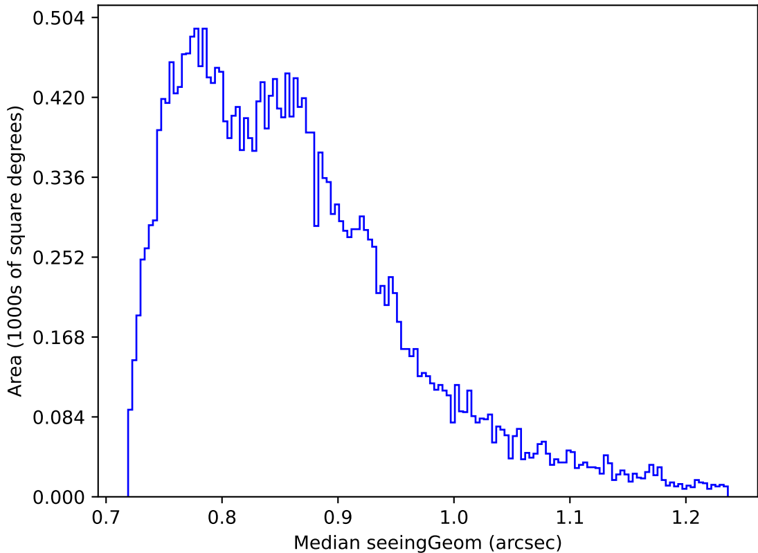
too_elab_r32_d3_griz_v3.4_10yrs Yr 1 all bands: Median seeingGeom
