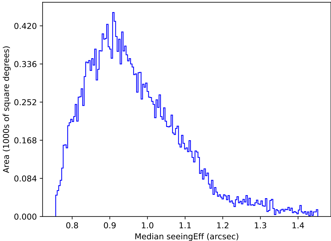
too_elab_r32_d3_griz_v3.4_10yrs Yr 1 z band: Median seeingEff
