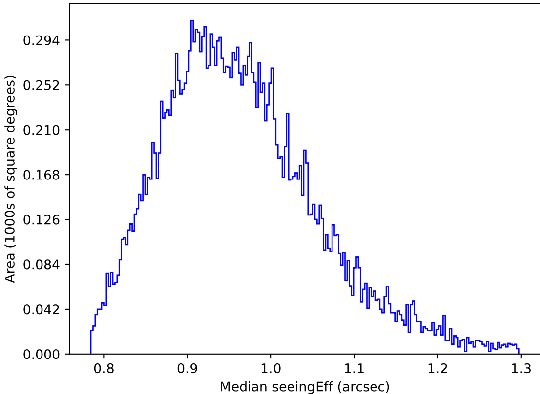
too_elab_r32_d3_griz_v3.4_10yrs Yr 1 y band: Median seeingEff
