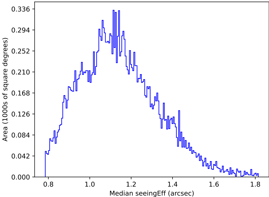
too_elab_r32_d3_griz_v3.4_10yrs Yr 1 u band: Median seeingEff
