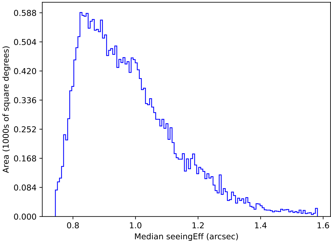
too_elab_r32_d3_griz_v3.4_10yrs Yr 1 r band: Median seeingEff
