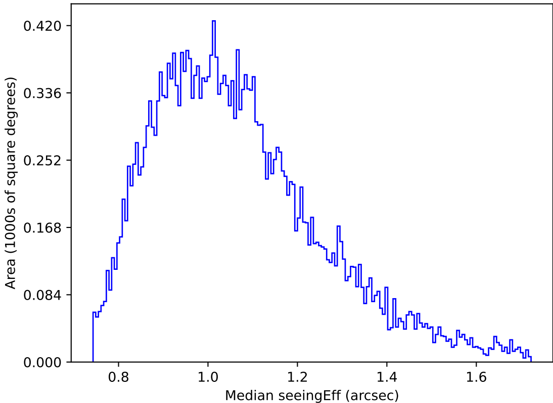
too_elab_r32_d3_griz_v3.4_10yrs Yr 1 g band: Median seeingEff
