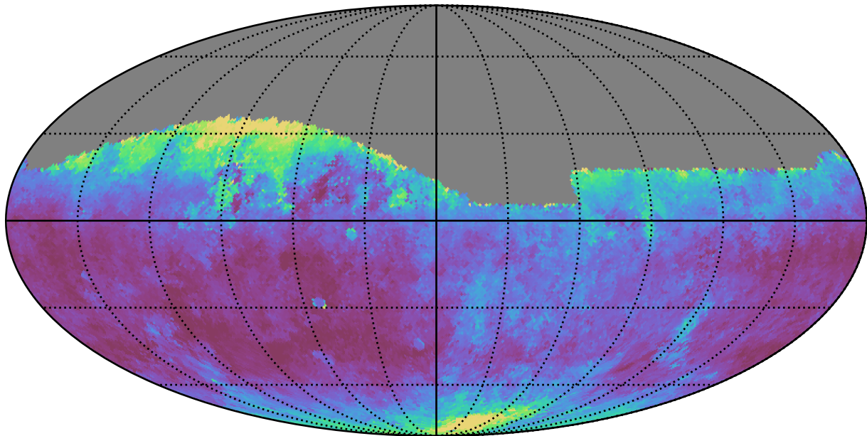
too_elab_r32_d3_griz_v3.4_10yrs Yr 1 all bands: Median seeingEff
