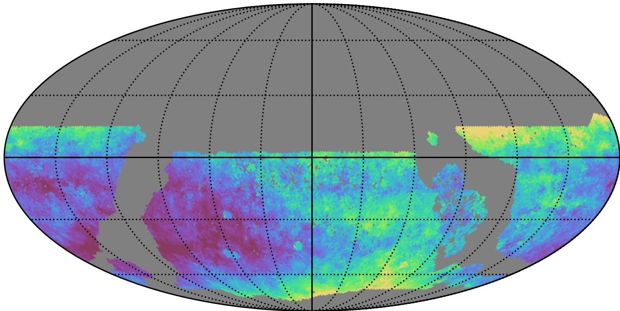
too_elab_r32_d3_griz_v3.4_10yrs WFD z band: Median seeingEff
