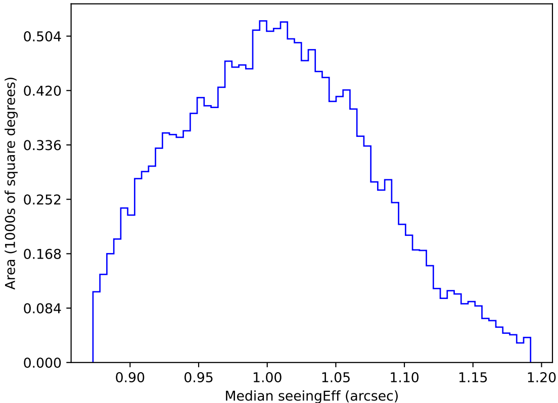
too_elab_r32_d3_griz_v3.4_10yrs WFD z band: Median seeingEff
