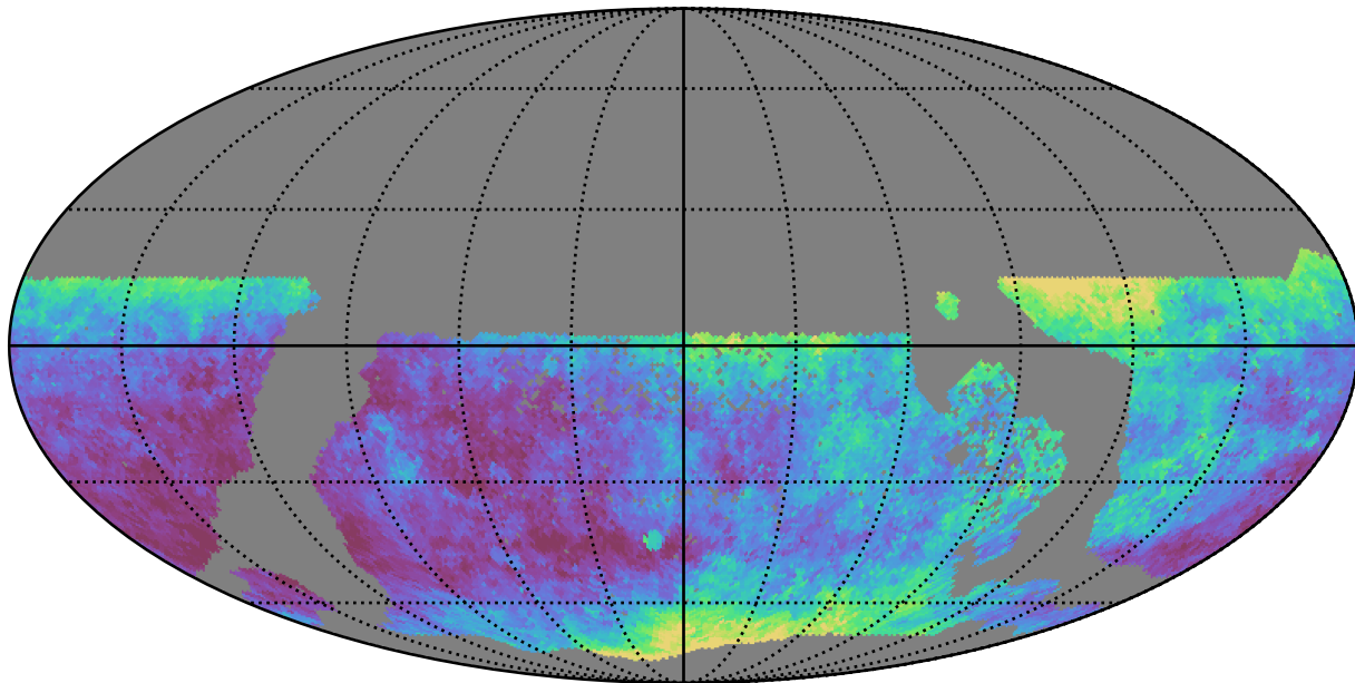
too_elab_r32_d3_griz_v3.4_10yrs WFD y band: Median seeingEff
