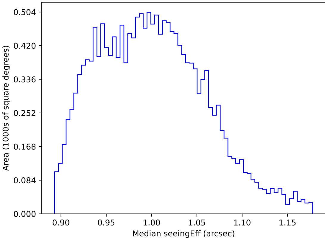
too_elab_r32_d3_griz_v3.4_10yrs WFD y band: Median seeingEff
