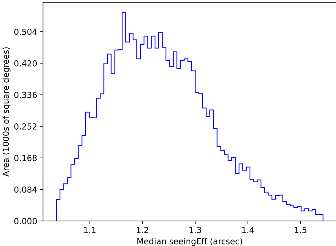
too_elab_r32_d3_griz_v3.4_10yrs WFD u band: Median seeingEff
