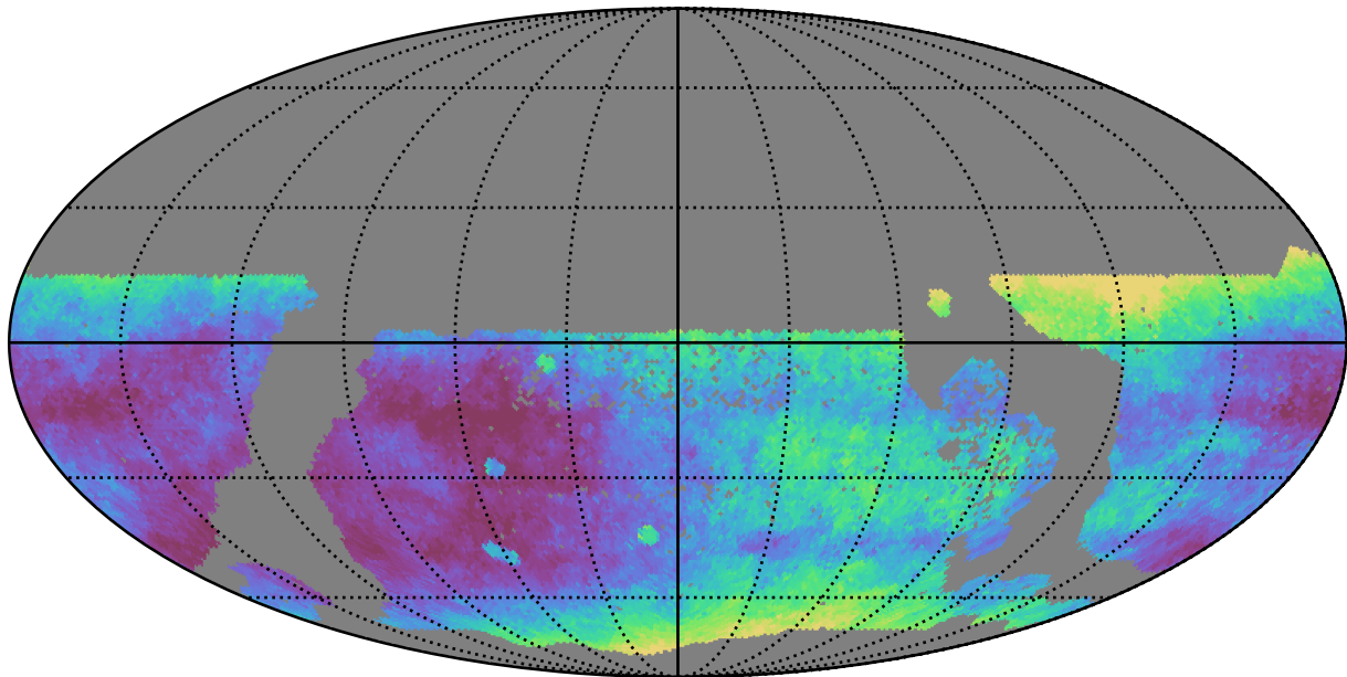
too_elab_r32_d3_griz_v3.4_10yrs WFD r band: Median seeingEff
