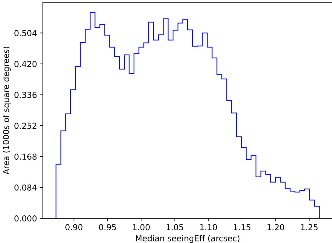
too_elab_r32_d3_griz_v3.4_10yrs WFD r band: Median seeingEff
