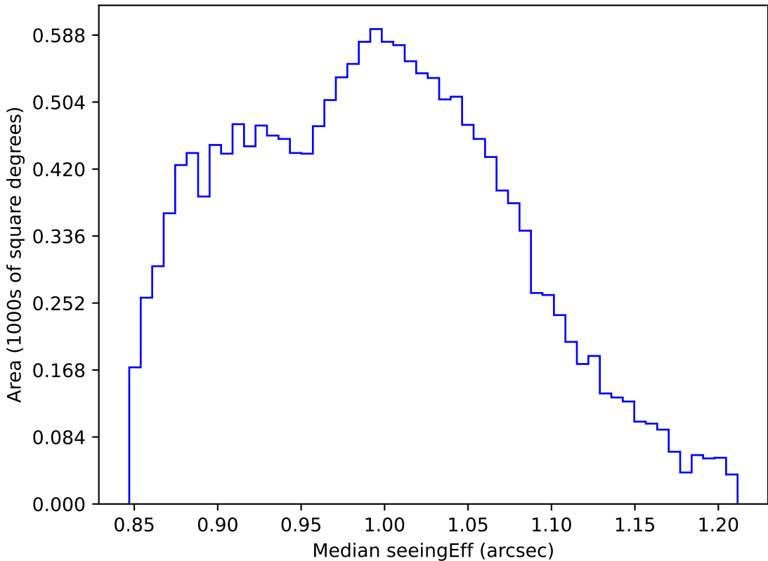
too_elab_r32_d3_griz_v3.4_10yrs WFD i band: Median seeingEff
