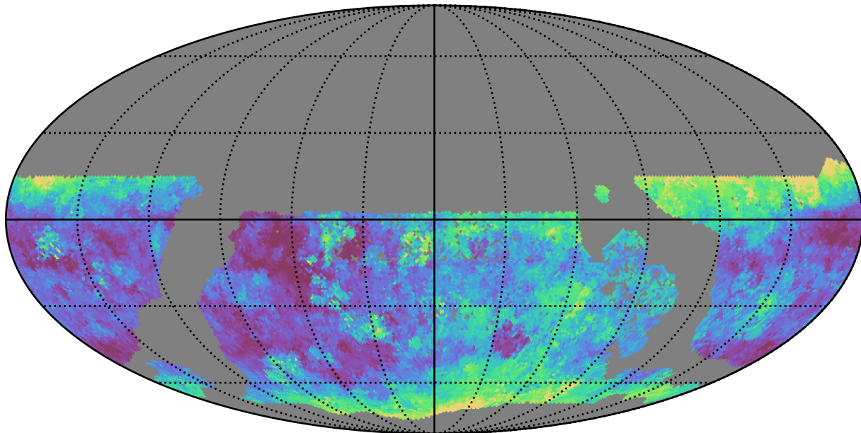
too_elab_r32_d3_griz_v3.4_10yrs WFD g band: Median seeingEff
