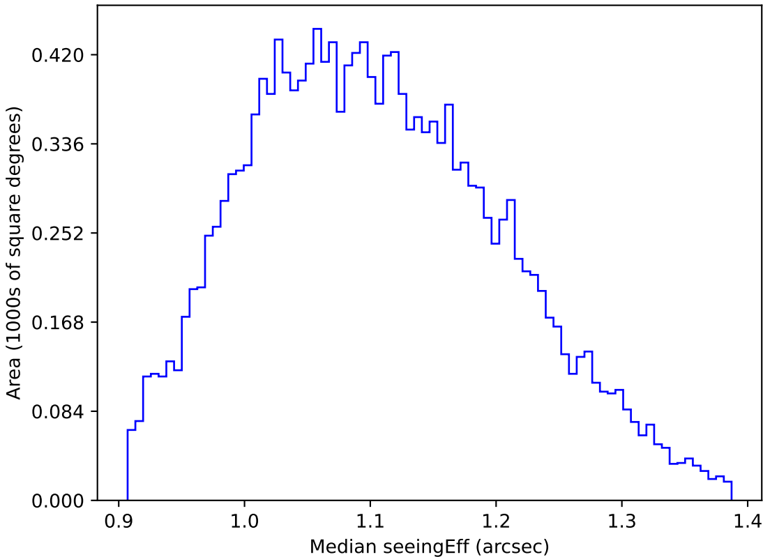
too_elab_r32_d3_griz_v3.4_10yrs WFD g band: Median seeingEff
