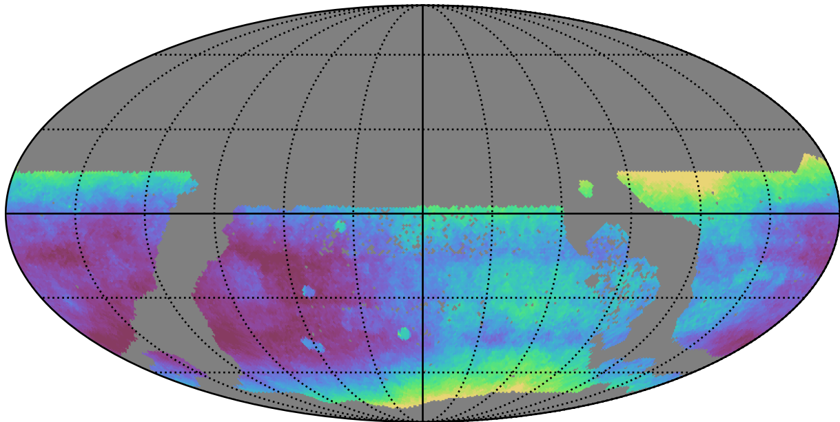
too_elab_r32_d3_griz_v3.4_10yrs WFD all bands: Median seeingEff
