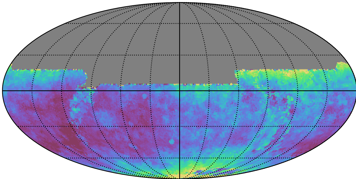
too_elab_r32_d3_griz_v3.4_10yrs All sky y band: Median seeingEff
