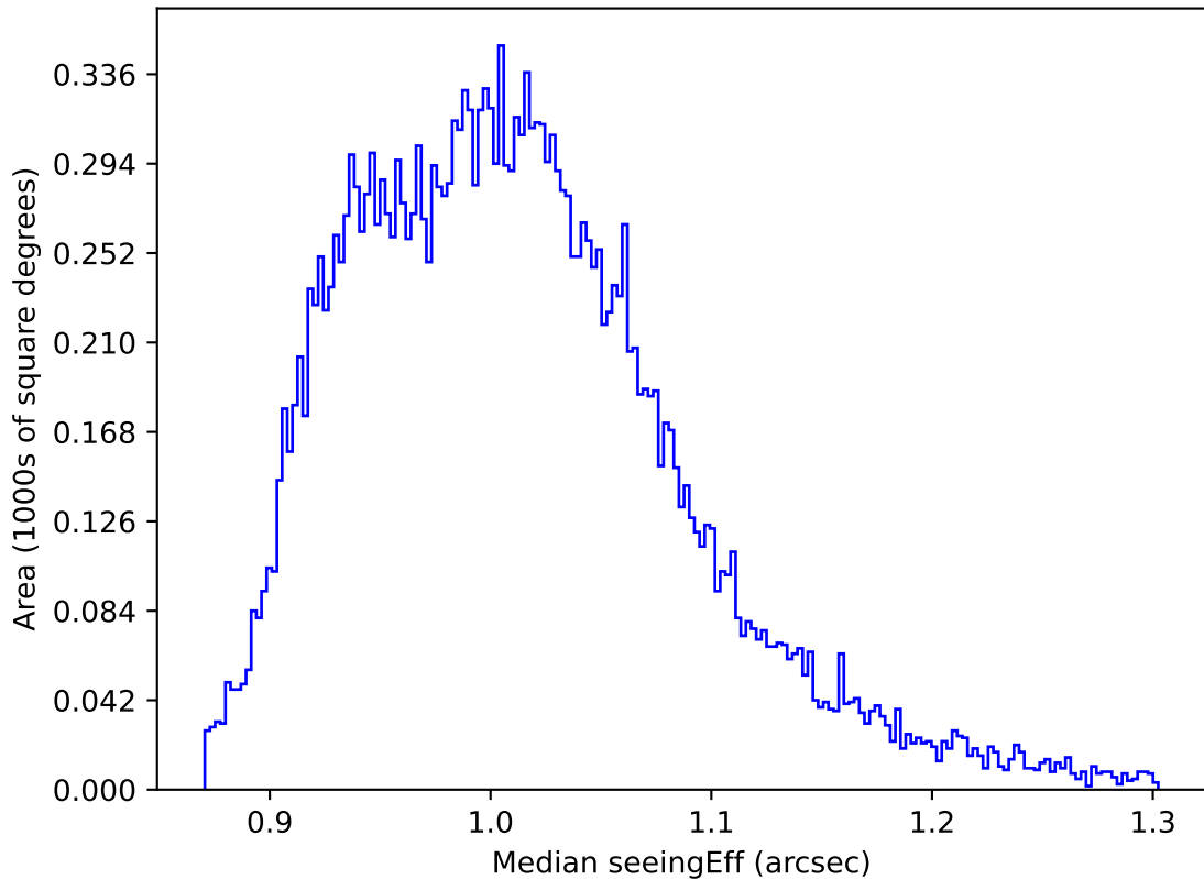
too_elab_r32_d3_griz_v3.4_10yrs All sky y band: Median seeingEff
