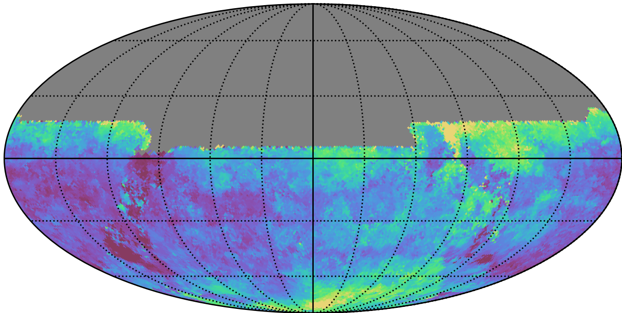
too_elab_r32_d3_griz_v3.4_10yrs All sky u band: Median seeingEff
