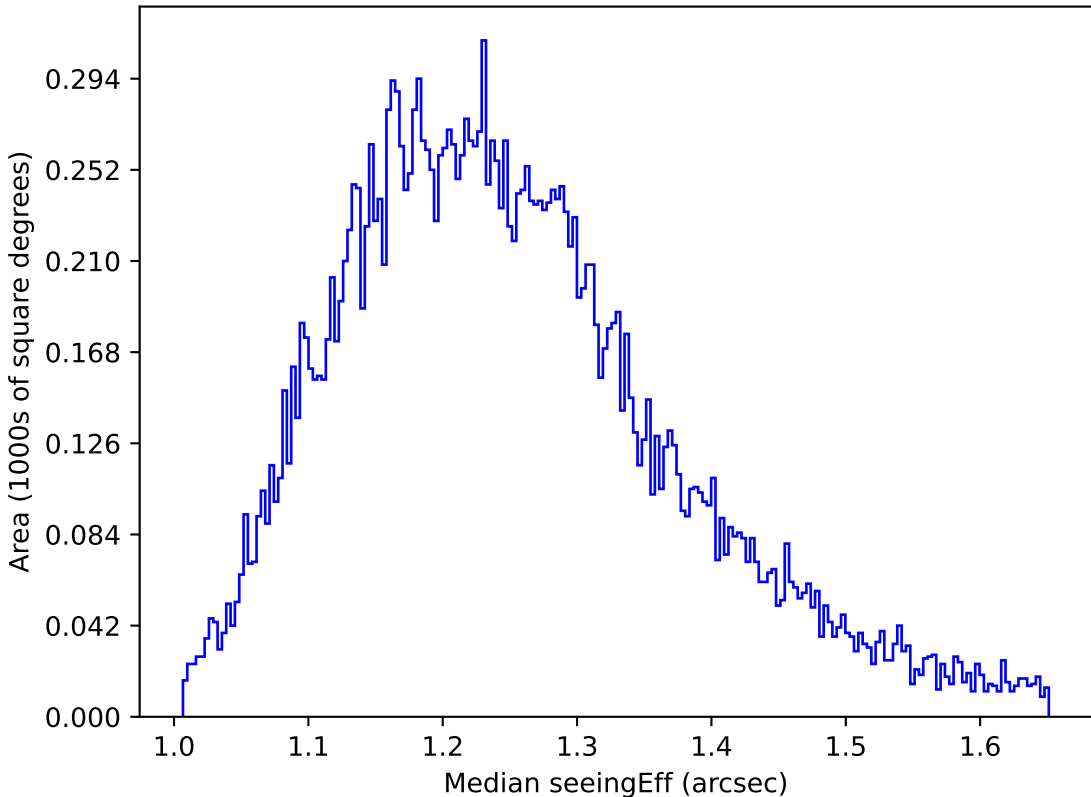
too_elab_r32_d3_griz_v3.4_10yrs All sky u band: Median seeingEff
